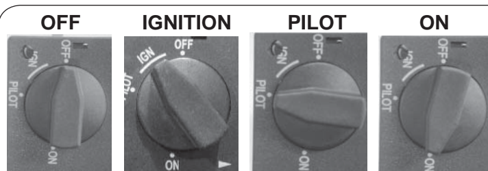
Ignition control knob - positions Fig. 23-1
